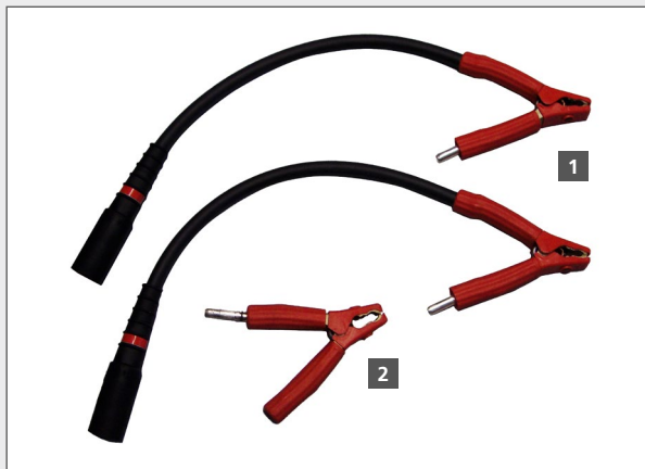
Figure 3: Pliers adapter set VLF CS-BB (3-phase)
