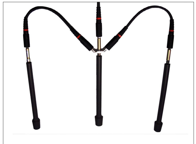
Figure 2: Installation of the 3-phase SF6 adapter set
